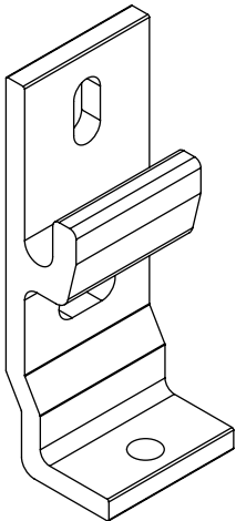
wall bracket
