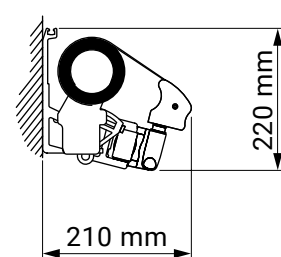
wall installation
