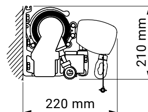
wall installation
