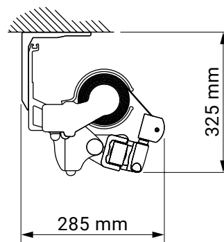
ceiling installation
