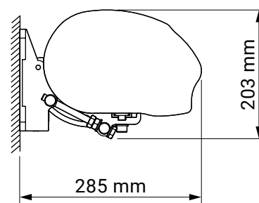
wall installation
