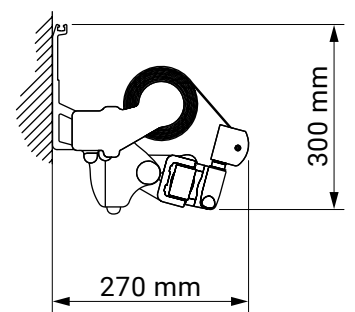
wall installation
