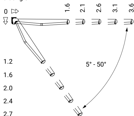
tilt angle
