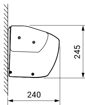
wall installation
