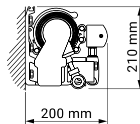
wall installation
