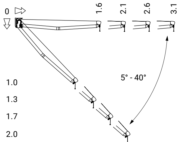
tilt angle
