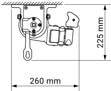
ceiling installation
