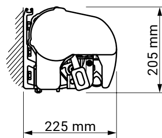
wall installation
